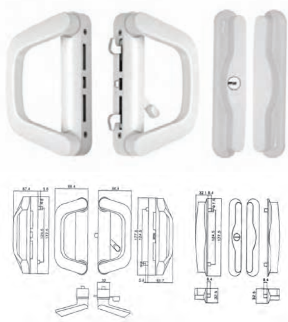
SGWSL-SGS304 Sliding Door Lock With One Side Thumbturn (Double Leaf)
