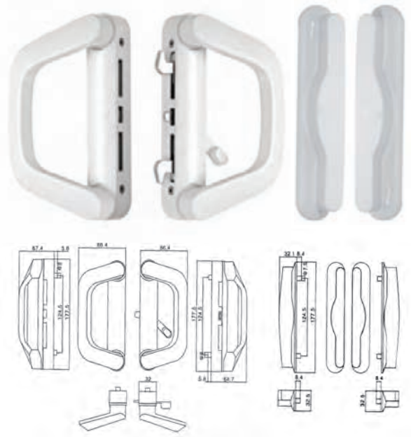
SGWSL-SGS304 Sliding Door Lock With One Side Thumbturn (Double Leaf)
