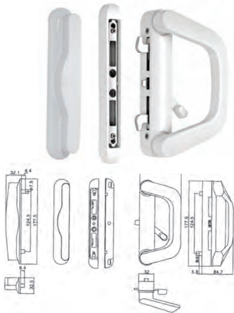
SGWSL-SGS303 Sliding Door Lock With One Side Thumbturn (Single Leaf)
