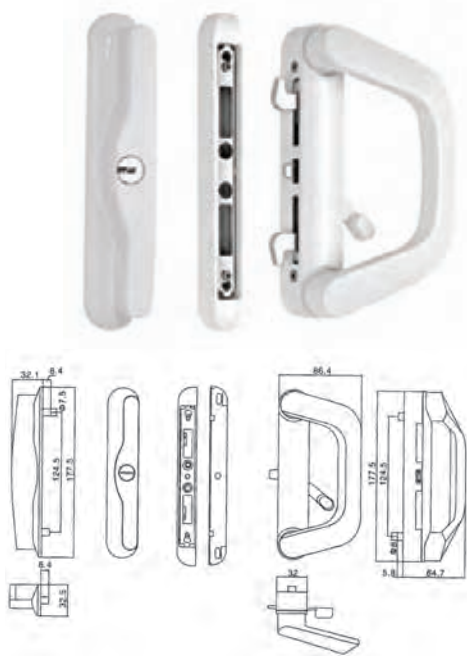
SGWSL-SGS303 Sliding Door Lock With One Side Thumbturn (Single Leaf)
